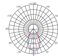
Luminous Intensity Unit : cd/klm Type V
